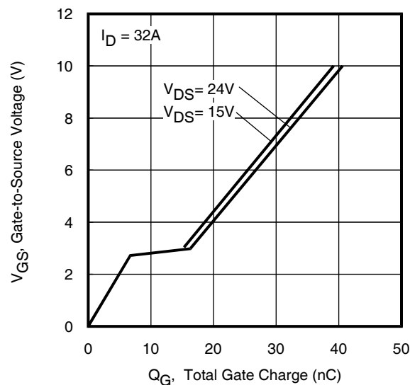
Fig 6. Typical Gate Charge vs. Drain-to-Source Voltage
