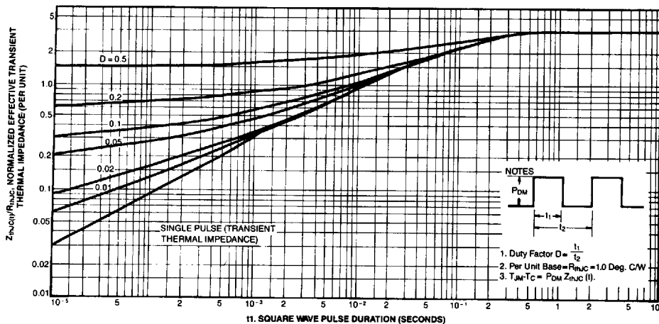
11. SQUARE WAVE PULSE DURATION (SECONDS) MAXIMUM EFFECTIVE TRANSIENT THERMAL IMPEDANCE JUNCTION-TO-CASE V_{GS} PULSE DURATION
