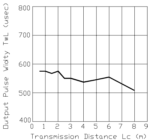
Fig.-6 Output Pulse Length vs. Arrival Distance
