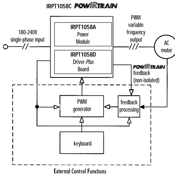
Figure 2. The IRPT1058C POWIRTRAIN within a motor control system
