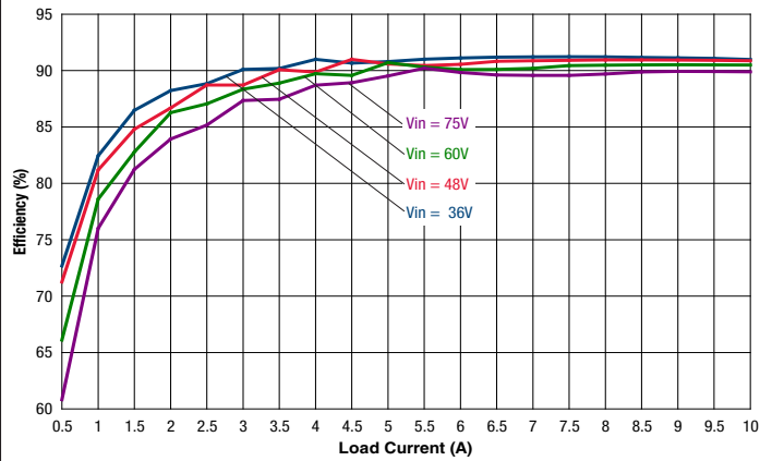
Efficiency vs. Line Voltage and Load Current @ 25°C – Vin = 36V-75V
