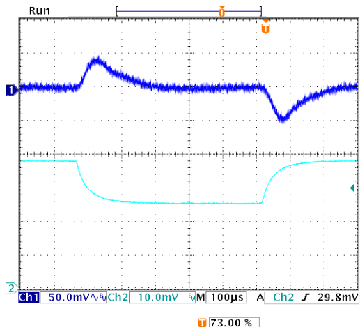
Step Load Transient Response (Vin=48V, Vout=nom., Iout=50-75-50% of full load, Cload=1 uF ceramic II 10uF tantulum, Ta=+25°C., ScopeBW=20MHz Ch1=5Vo, Ch2=Io 2amps/div)
