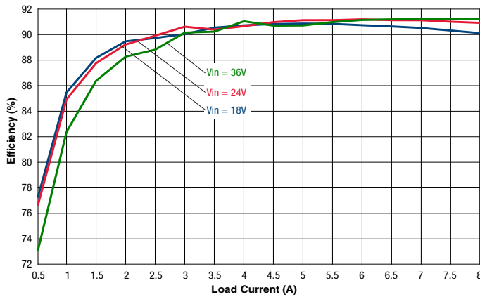
Efficiency vs. Line Voltage and Load Current @ 25°C – Vin = 18V-36V
