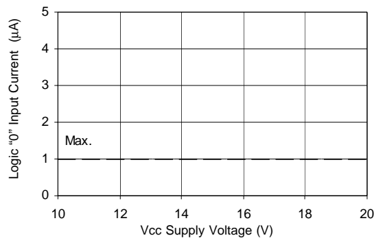
Figure 17B. Logic "0" Input Current vs. Voltage
