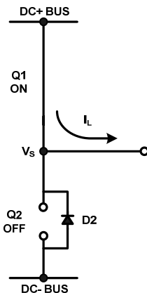
Figure 6: Q1 conducting
