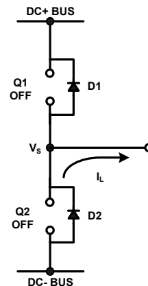
Figure 7: D2 conducting
