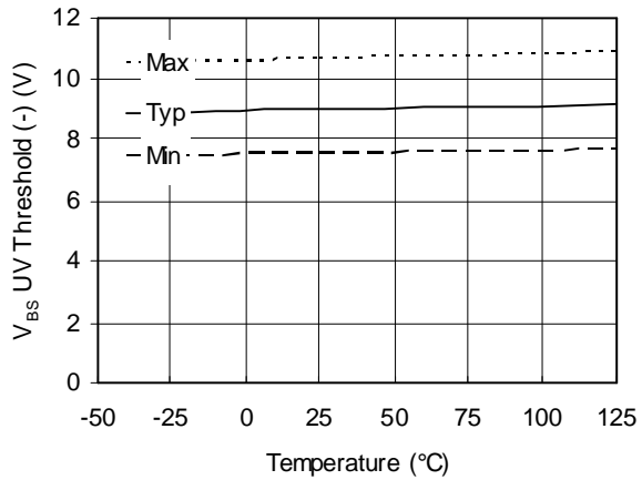
Figure 26A. V_{BS} UV Threshold (-) vs. Temperature
