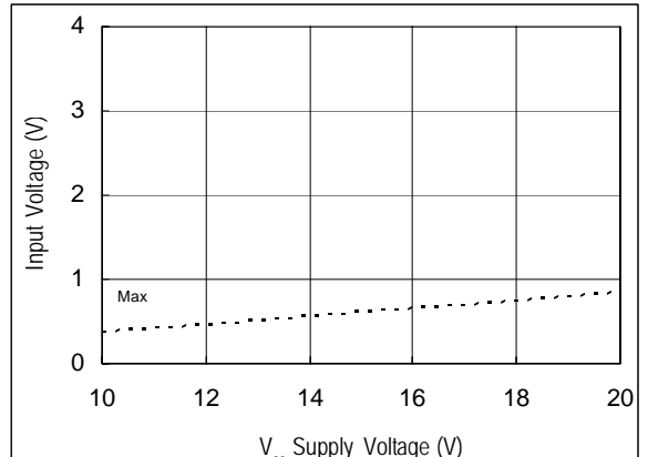
Figure 8B. Logic "0" Input Voltage vs. Supply Voltage
