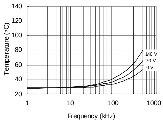
Figure 23. IRS2304 vs. Frequency (IRFBC20), R_{gate}=33\Omega , V_{CC}=15V
