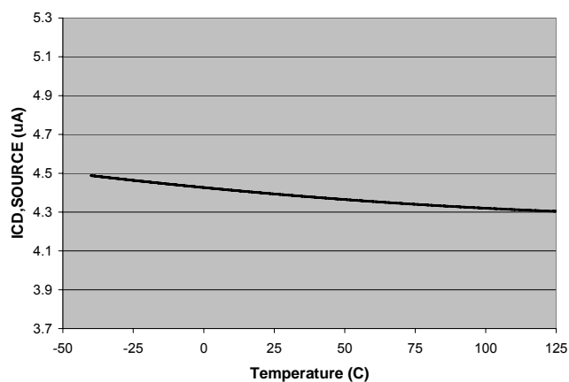
Figure 36: I_{CD,SOURCE} vs. temperature
