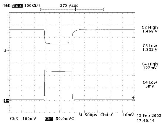
Figure 25 - 60A Load dynamic with 20A/μs slew rate. Ch4: Output current, sensed through 2mΩ resistor, 25A/div. Ch3: Output voltage, DC offset 1.3V, 100mV/div.
