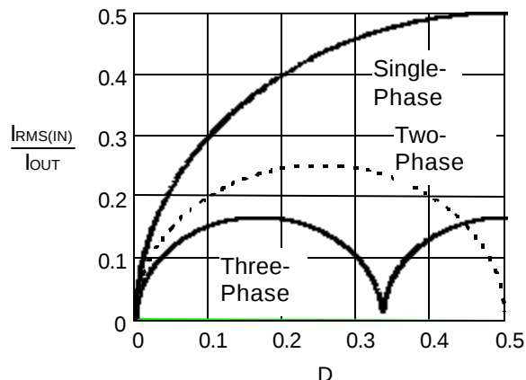
Figure 12 - Normalized input RMS current vs. duty cycle.
