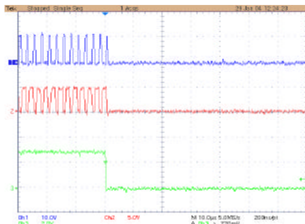
Figure 16 - Shut Down the output by pulling down the soft-start pin
