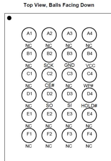
TFBGA-24 (Package: JG)
