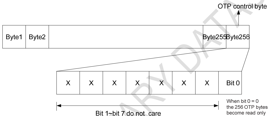
Figure 28. OTP area
