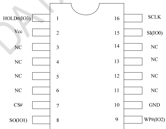
16-Pin SOIC
