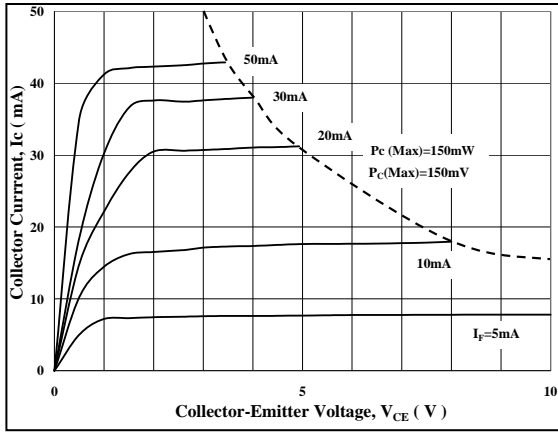
Fig 7 Collector Current vs Collector-Emitted Voltage
