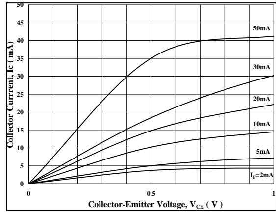
Fig 8 Collector Current vs Low Collector-Emitted Voltage
