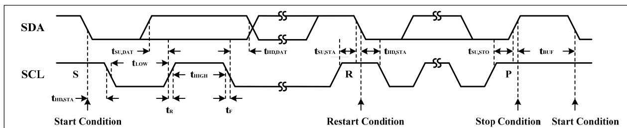
Figure 13 Interface timing
