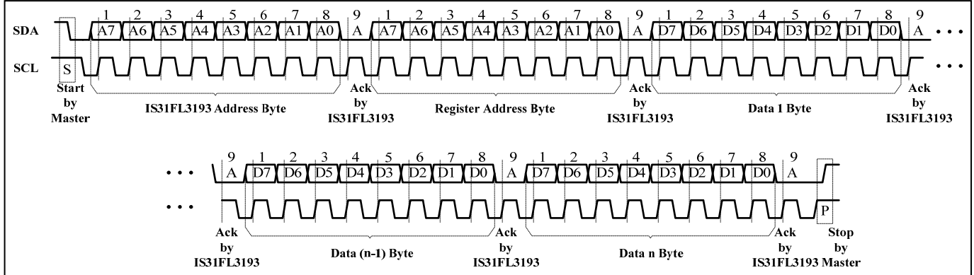
Figure 5 Writing to IS31FL3193 (Automatic Address Increment)
