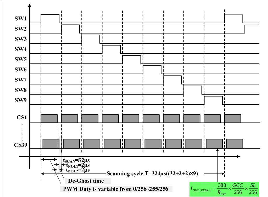
Figure 11 Scanning Timing
