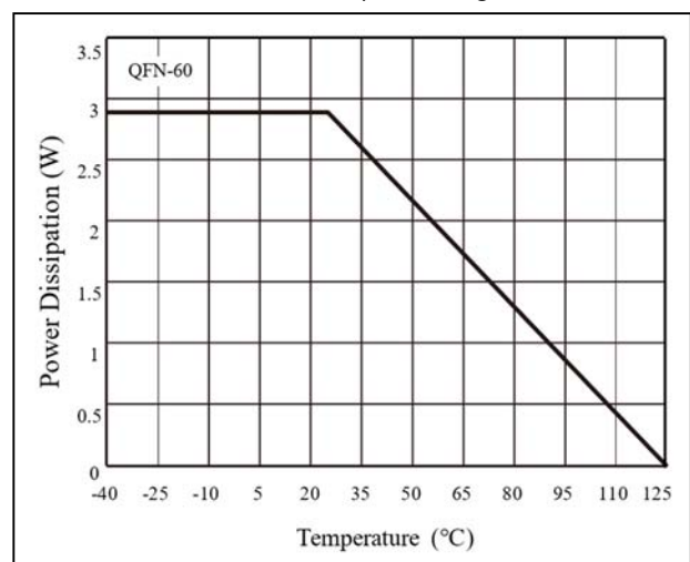
Figure 20 Dissipation Curve
