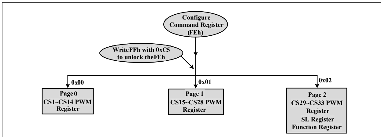
Figure 14 Register Pages (For I2C Mode Only)
