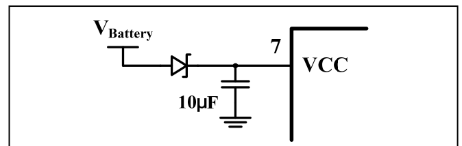
Figure 67 Capacitor For Latch Status
