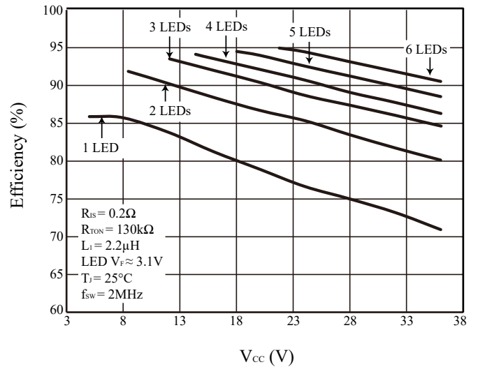
Figure 17 Efficiency vs. V_{CC}
