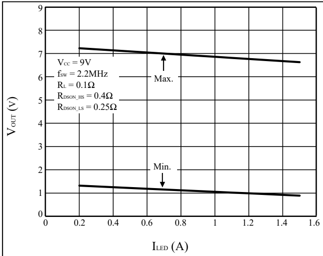
Figure 46 Minimum and Maximum Output Voltage versus LED Current (minimum t_{ON}=80ns and minimum t_{OFF}=90ns )
