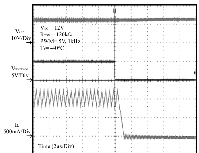
Figure 25 PWM Off
