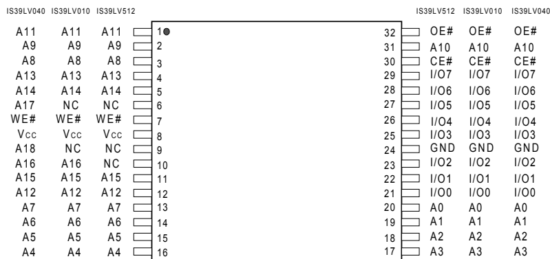
32-Pin VSOP
