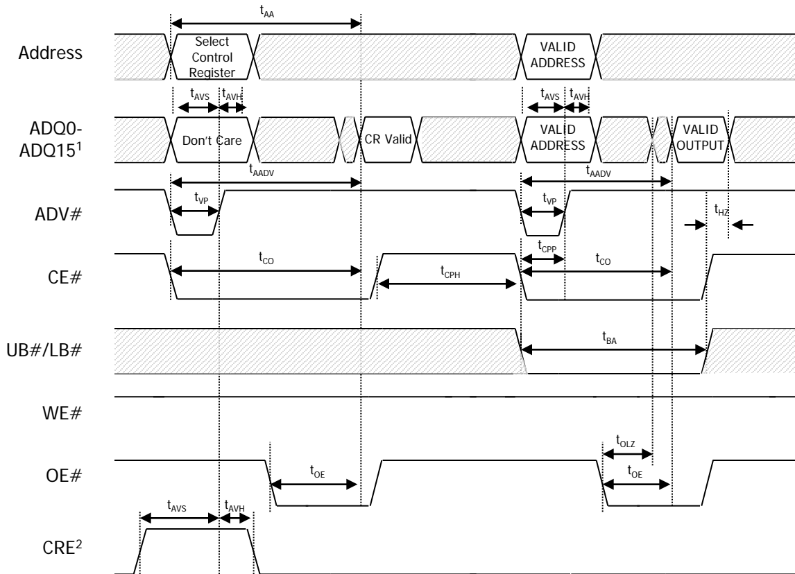
Figure 8: Configuration Register READ – Asynchronous Mode Followed by DATA READ
