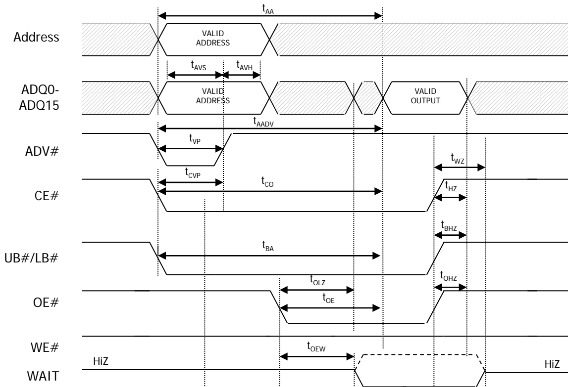
Figure 19: Asynchronous READ
