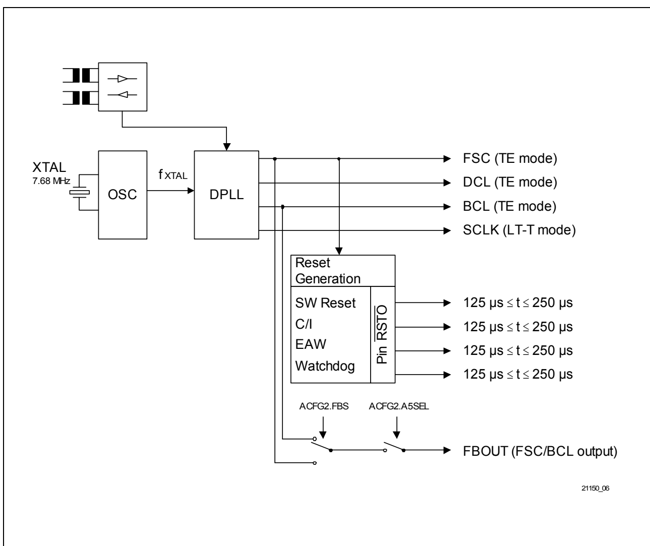
Figure 34 Clock System of the ISAC-SX
