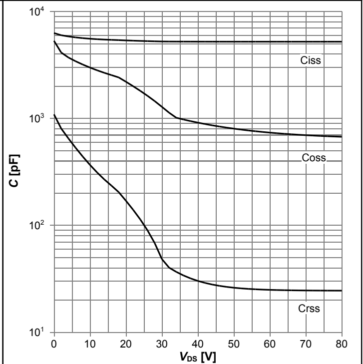
Diagram 12: Typ. capacitances
