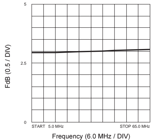
NOISE FIGURE
