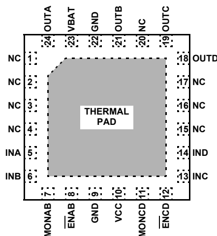
ISL1541 [24 Ld QFN (6mm x 6mm)] TOP VIEW
