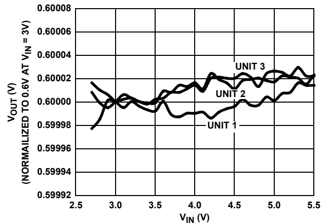
FIGURE 4. LINE REGULATION
