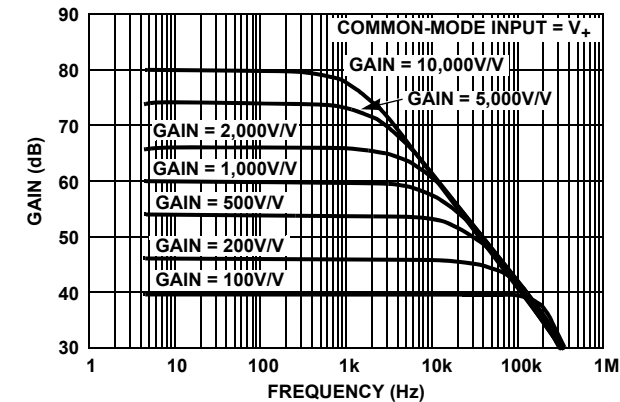
FIGURE 1. ISL28270, ISL28470 FREQUENCY RESPONSE vs CLOSED LOOP GAIN, V_{CM} = V_+ = 5V
