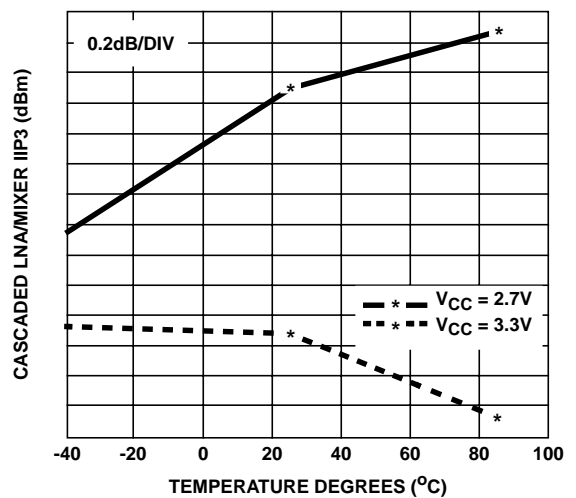
FIGURE 30. INPUT IIP3 HIGH GAIN MODE
