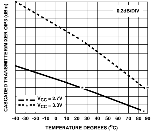
FIGURE 38. OUTPUT IP3
