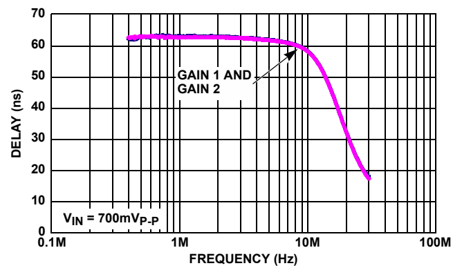
FIGURE 16. COMPOSITE GROUP DELAY
