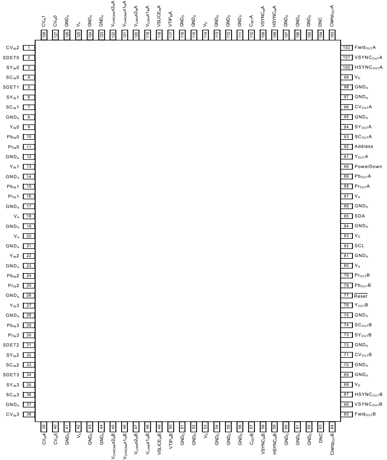
ISL59450 (128 LD MQFP) TOP VIEW
