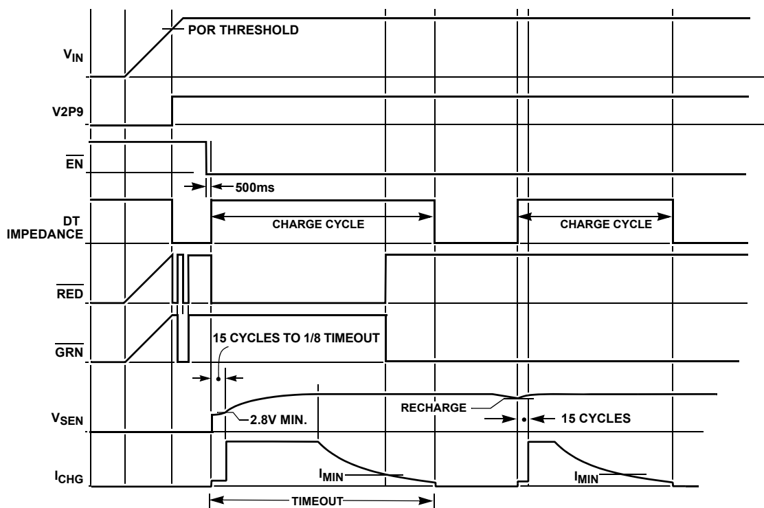
FIGURE 6. OPERATION WAVEFORMS
