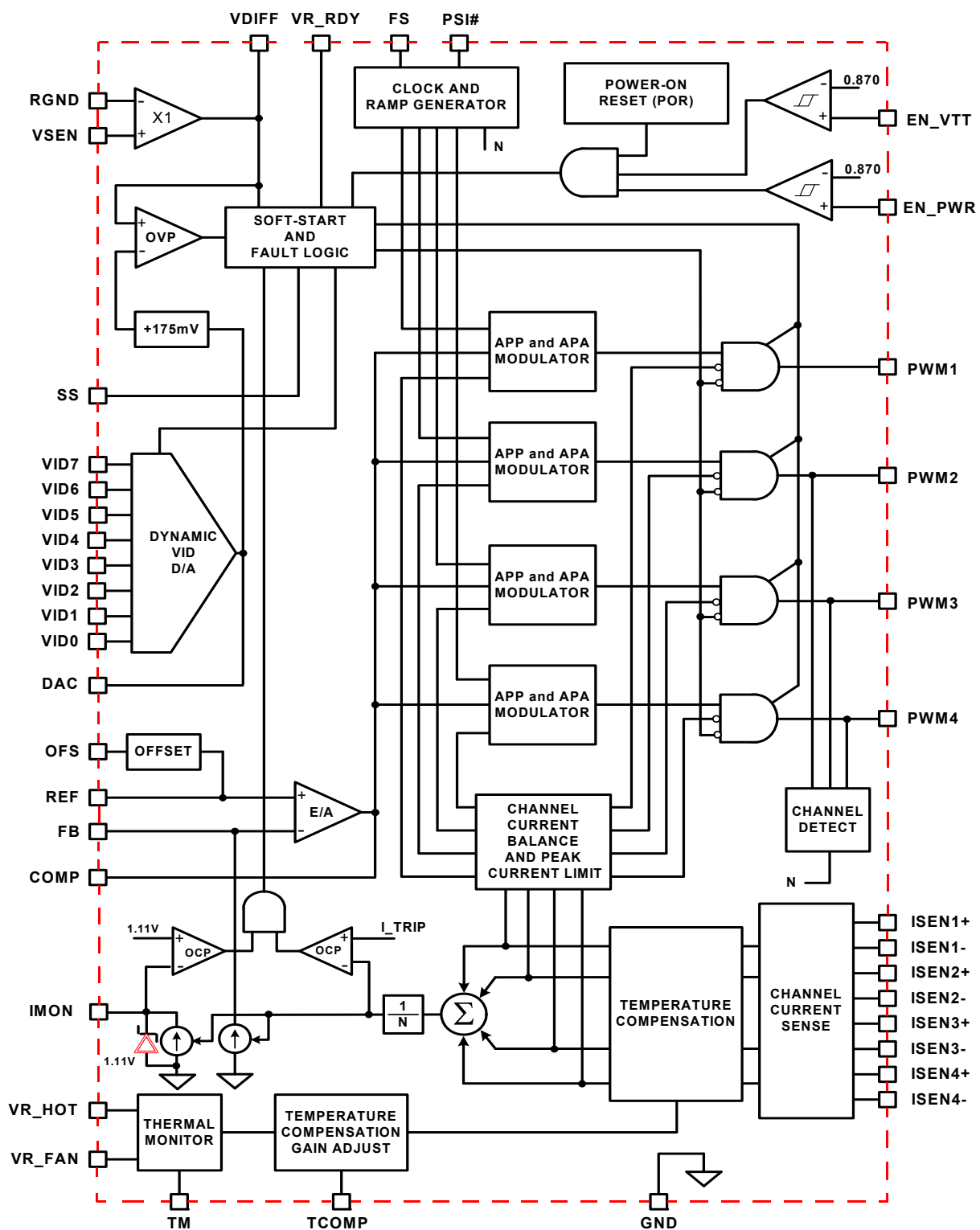
FIGURE 1. BLOCK DIAGRAM
