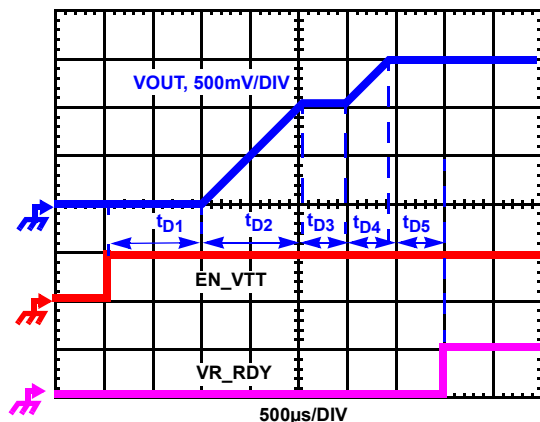
FIGURE 13. SOFT-START WAVEFORMS
