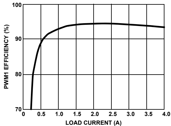
FIGURE 11. PWM1 EFFICIENCY vs LOAD (3.3V), V IN = 5V
