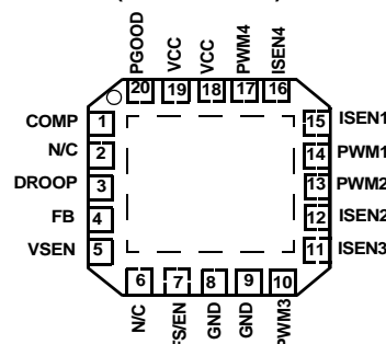
ISL6558 (20 LEAD QFN) TOP VIEW
