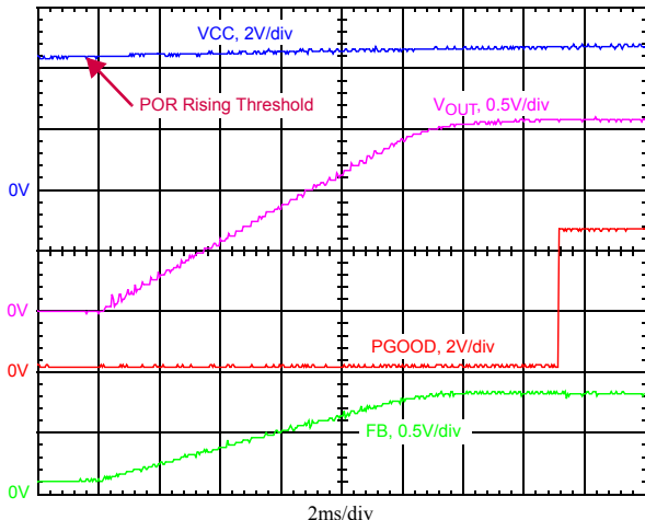
FIGURE 3. SOFT-START WAVEFORMS
