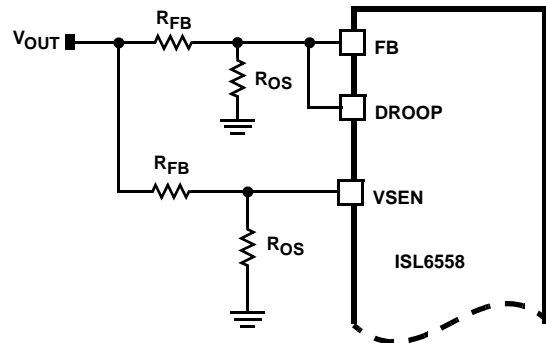
FIGURE 8. VSEN RESISTOR DIVIDER CONFIGURATION
