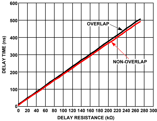
FIGURE 3. DELAY TIME vs RESISTANCE
