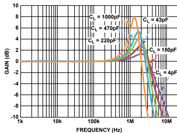
FIGURE 38. FREQUENCY RESPONSE vs C_L ( \pm 2.5V )
