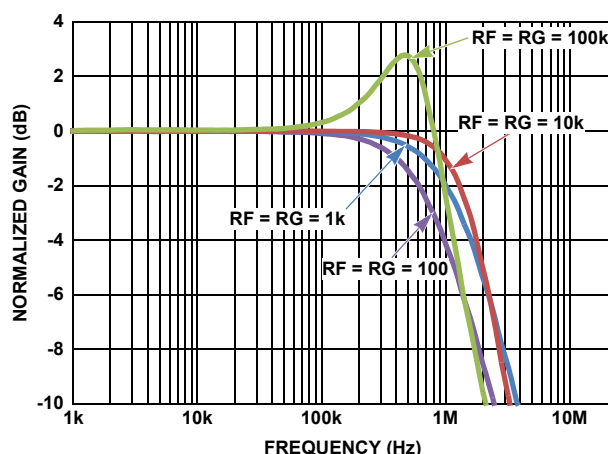
FIGURE 34. FREQUENCY RESPONSE vs FEEDBACK RESISTANCE ( \pm 18.0V )
