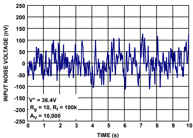
FIGURE 22. INPUT NOISE VOLTAGE (0.1Hz TO 10Hz)
