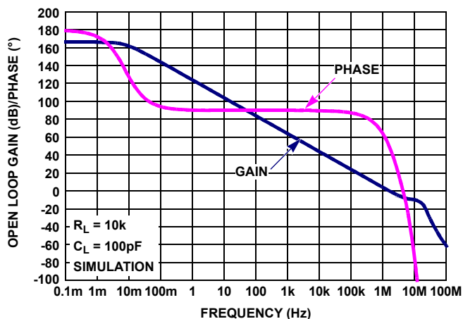
FIGURE 26. OPEN LOOP FREQUENCY RESPONSE ( R_L = 10k\Omega , C_L = 100pF )
