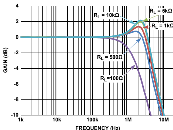
FIGURE 36. FREQUENCY RESPONSE vs R_L ( \pm 5.0V )
