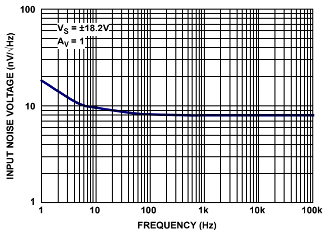
FIGURE 23. INPUT NOISE VOLTAGE SPECTRAL DENSITY
