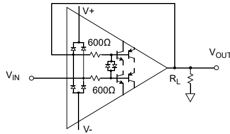
Figure 53. Input ESD Diode Current Limiting, Unity Gain
