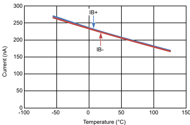
Figure 8. I_{BIAS} vs Temperature ( V_S = \pm 1.5V )
