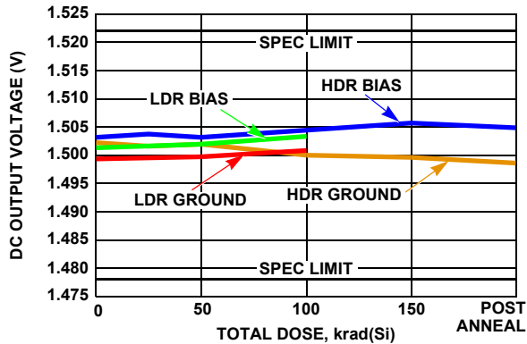
FIGURE 5. DC OUTPUT VOLTAGE, 1.5V_{OUT} , 3.6V_{IN} NO LOAD
