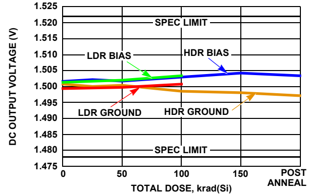
FIGURE 6. DC OUTPUT VOLTAGE, 1.5V_{OUT} , 3.6V_{IN} , 3A LOAD
