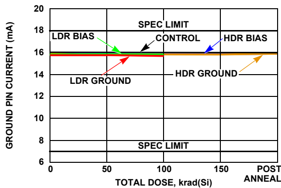
FIGURE 7. GROUND PIN CURRENT, 5.0V_{OUT} , 5.5V_{IN} , NO LOAD
