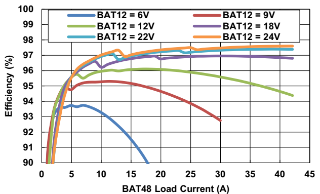
Figure 2. Boost Mode, DE Mode, Phase-Drop Enabled
