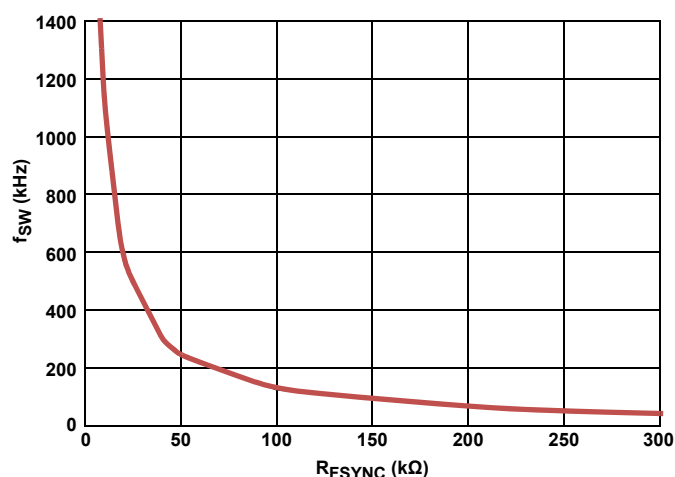
FIGURE 40. R_{\text{FSYNC}} vs f_{\text{SW}}
