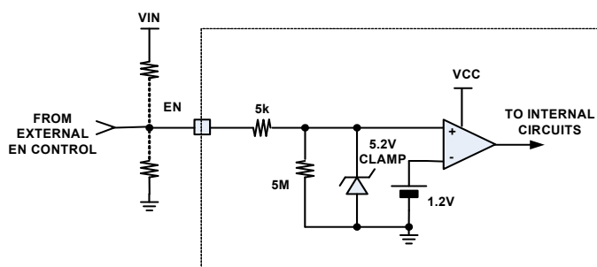
FIGURE 39. ENABLE BLOCK
