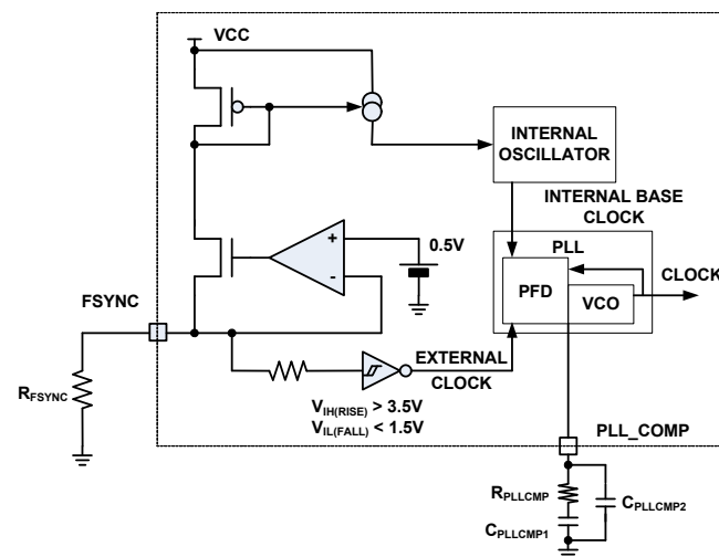
FIGURE 41. CLOCK GENERATOR AND EXTERNAL CLOCK SYNCHRONIZATION BLOCK
