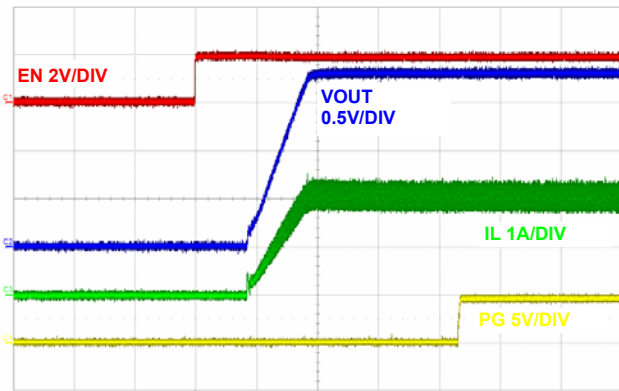
FIGURE 25. SOFT-START AT FULL LOAD, (2ms/DIV)
