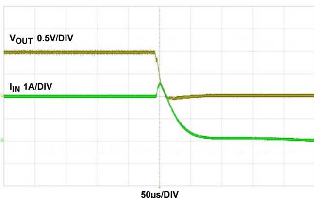
FIGURE 22. SHORT CIRCUIT AT 20A
