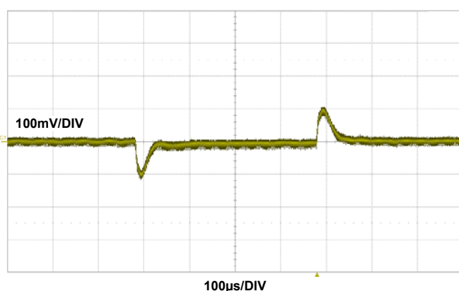
FIGURE 12. 1.5VOUT TRANSIENT RESPONSE, I_{OUT} = 0A TO 10A , f_{SW} = 400kHz , C_{OUT} = 2x10\mu F + 7x100\mu F CERAMIC CAPACITOR, CFF = 6.8nF
