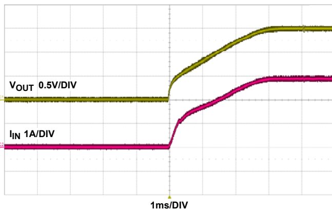
FIGURE 20. START-UP AT 20A
