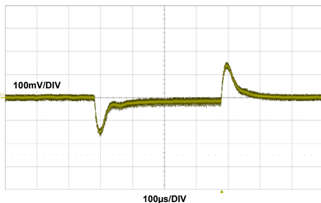
FIGURE 14. 2.5VOUT TRANSIENT RESPONSE, I_{OUT} = 0A TO 10A , f_{SW} = 500kHz , C_{OUT} = 2x10\mu F + 7x100\mu F CERAMIC CAPACITOR, CFF = 6.8nF
