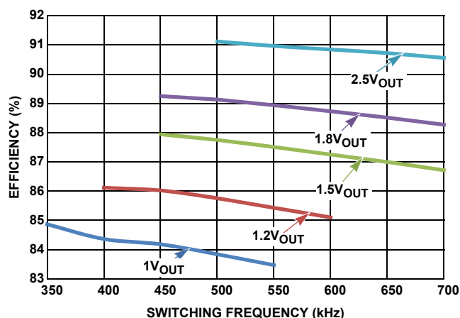
FIGURE 10. EFFICIENCY vs SWITCHING FREQUENCY AT V_{IN} = 12V (PARALLEL SINGLE OUTPUT, AS SHOWN IN Figure 24 AT 12VIN) AND I_{OUT} = 18A FOR VARIOUS OUTPUT VOLTAGES
