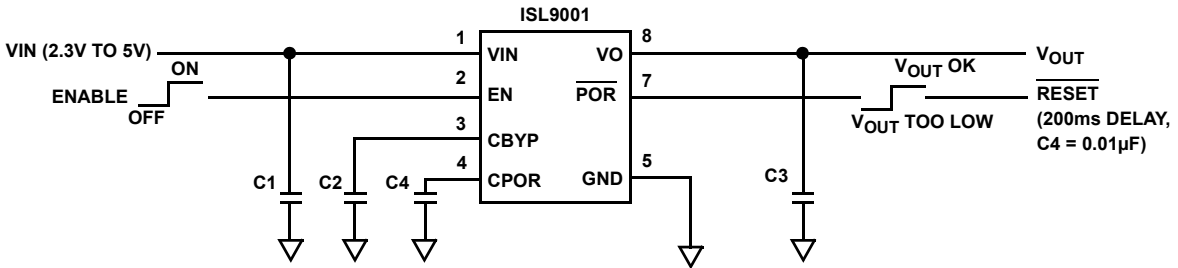
C1, C3: 1 \mu F X5R CERAMIC CAPACITOR C2: 0.01 \mu F X7R CERAMIC CAPACITOR C4: 0.01 \mu F X7R CERAMIC CAPACITOR
