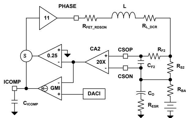
FIGURE 27. CHARGE CURRENT LIMIT LOOP
