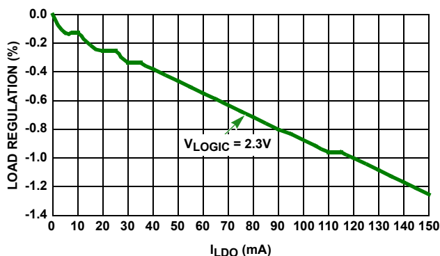
FIGURE 9. LOGIC LDO LOAD REGULATION
