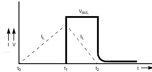
Figure 15. Avalanche Current and Voltage Waveforms
