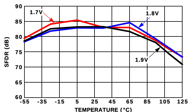
FIGURE 24. SFDR PERFORMANCE vs TEMPERATURE (CAL DONE AT +25°C)
