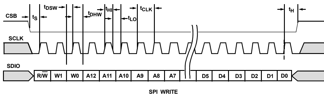
FIGURE 35. SPI WRITE
