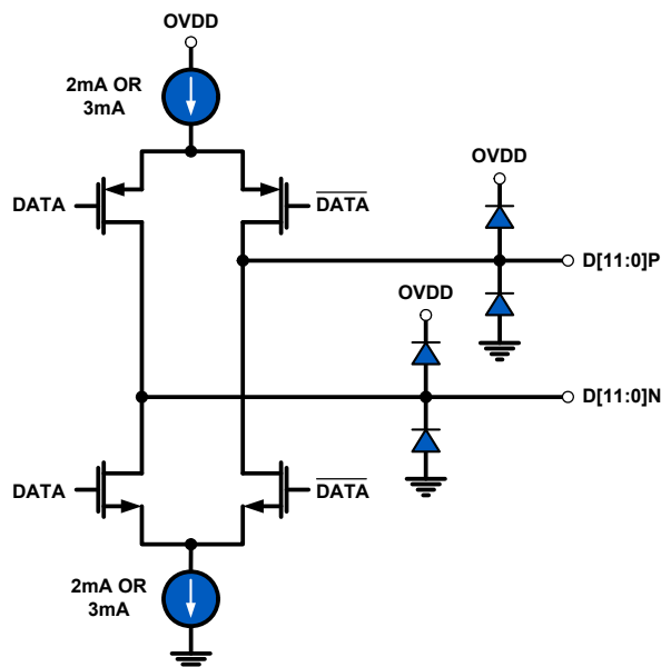
FIGURE 45. LVDS OUTPUTS
