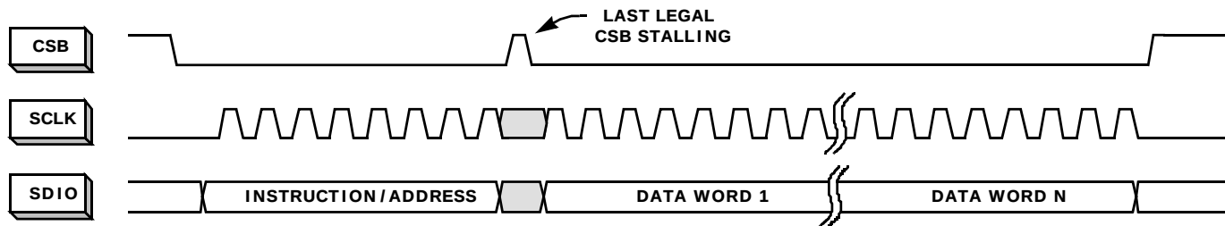
FIGURE 38. N-BYTE TRANSFER
