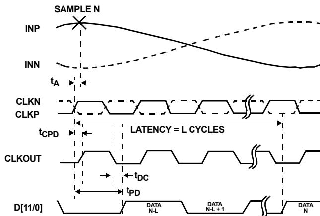
FIGURE 2B. SDR
