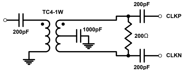
FIGURE 29. RECOMMENDED CLOCK DRIVE
