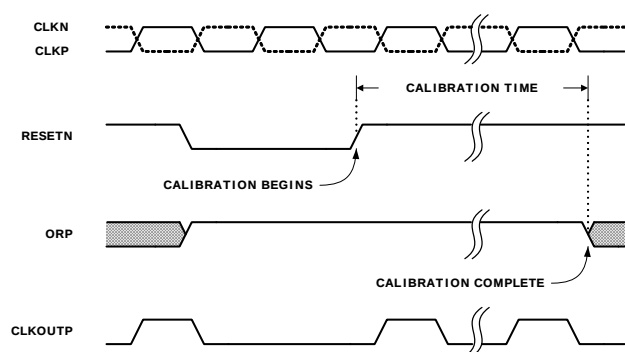
FIGURE 22. CALIBRATION TIMING
