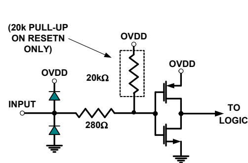
FIGURE 44. DIGITAL INPUTS
