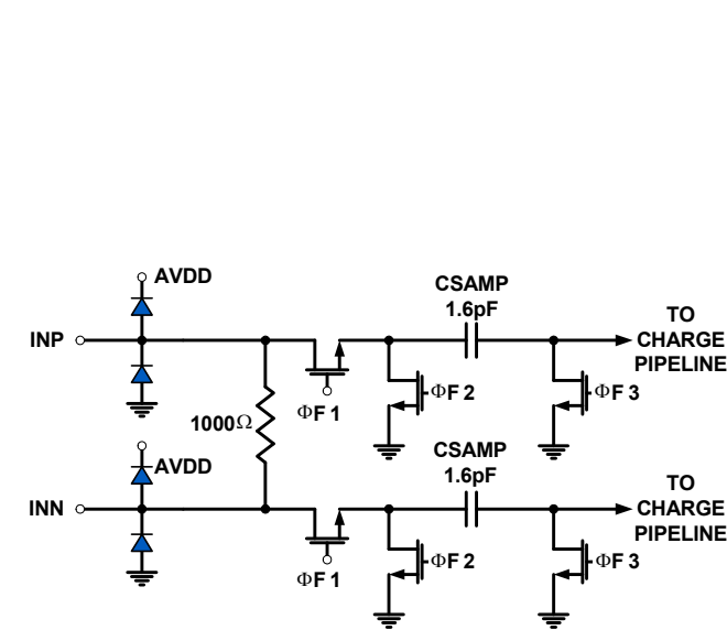
FIGURE 41. ANALOG INPUTS
