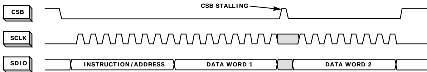
FIGURE 37. 2-BYTE TRANSFER
