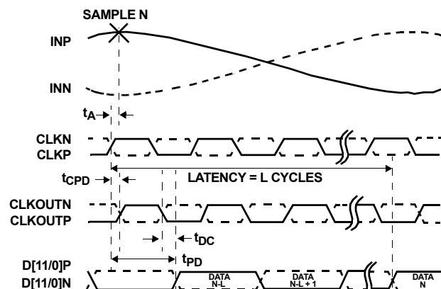
FIGURE 1B. SDR
