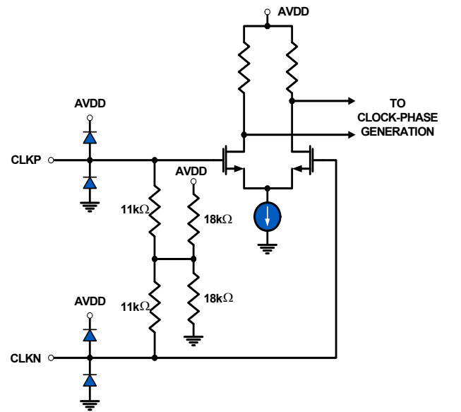
FIGURE 42. CLOCK INPUTS
