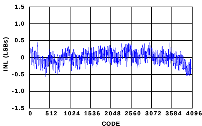
FIGURE 11. INTEGRAL NONLINEARITY
