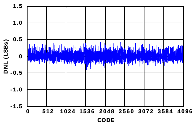
FIGURE 10. DIFFERENTIAL NONLINEARITY
