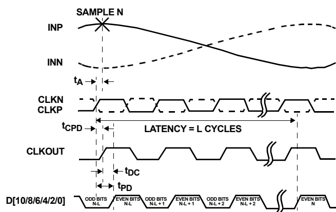
FIGURE 2A. DDRx
