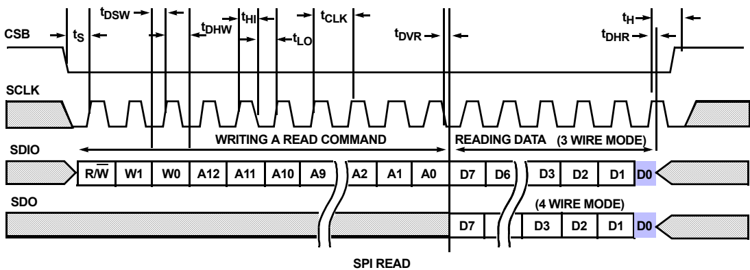
FIGURE 36. SPI READ
