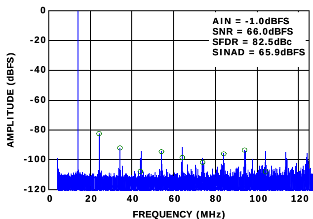
FIGURE 14. SINGLE-TONE SPECTRUM @ 10MHz
