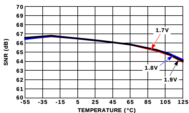
FIGURE 23. SNR PERFORMANCE vs TEMPERATURE (CAL DONE AT +25°C)
