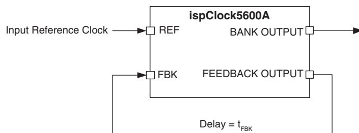
Figure 1-27. External Feedback Mode and Timing Relationships (Input, Output and Feedback Use the Same Logic Standard)
