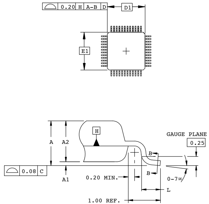
DETAIL "A"
