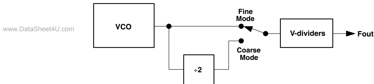
Figure 1-24. Additional Factor-of-2 Division in Coarse Mode
