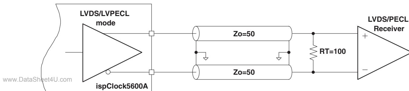
Figure 1-23. Configuration for LVDS and LVPECL Output Modes
